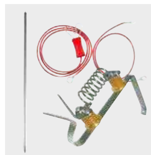
Earth stake 1.5 m (125H15017-1), fence connection kit (125H15522), lightning protection choke (125H15482)
